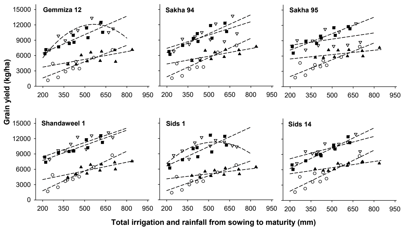
Figure 2. Grain yield in relation to total seasonal water input from both irrigation and rainfall from sowing to maturity for six wheat cultivars at Nubaria ( \blacktriangle ), Al Mataenah ( \blacksquare ), Sids ( \nabla ) and Ismailia ( \circ ). The dashed lines are drawn from the estimated equations in Table 9.
