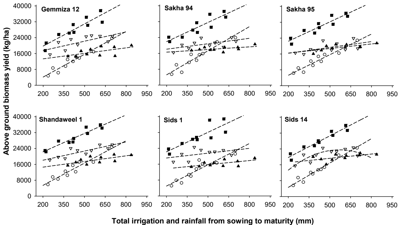
Figure 3. Above-ground biomass yield in relation to the total seasonal water input from both irrigation and rainfall from sowing to maturity for six wheat cultivars at Nubaria (▲), Al Mataenah (■), Sids (▽) and Ismailia (○). The dashed lines are drawn from the estimated equations in Table 10.
